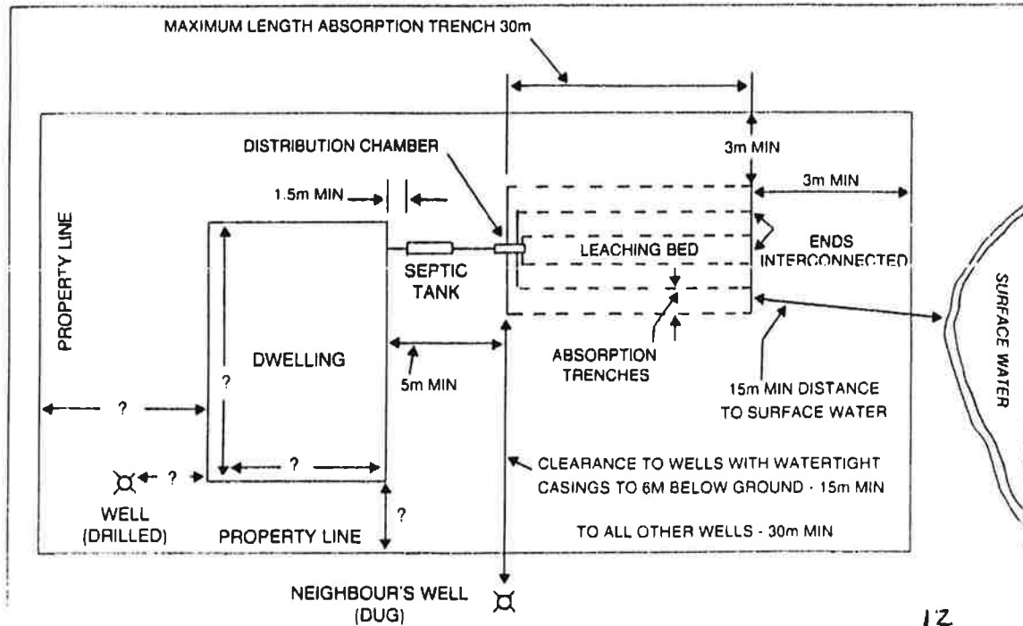
TYPICAL ARRANGEMENT OF A SEPTIC TANK SYSTEM METRIC MEASUREMENTS
